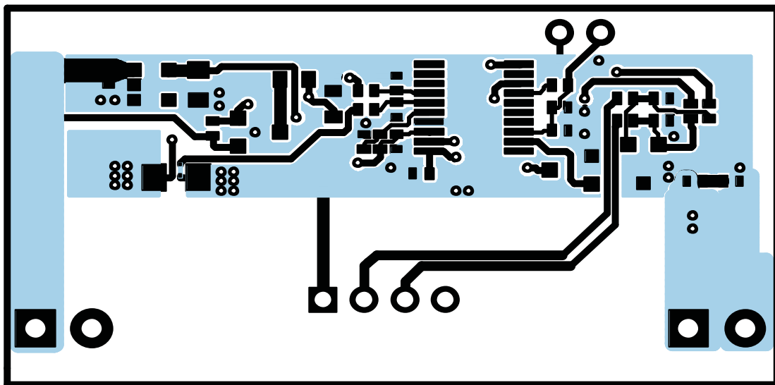
Figure 3. Top Layer
