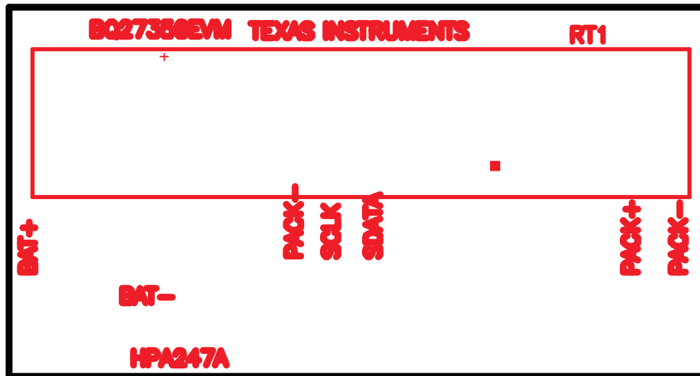
Figure 1. bq27350EVM-001 Layout (Silk Screen)
