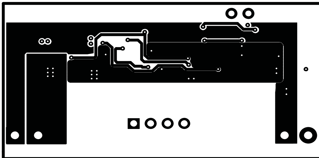
Figure 4. Bottom Layer
