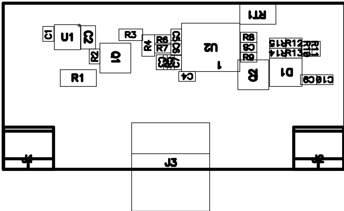
Figure 2. Top Assembly
